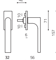
K269B
